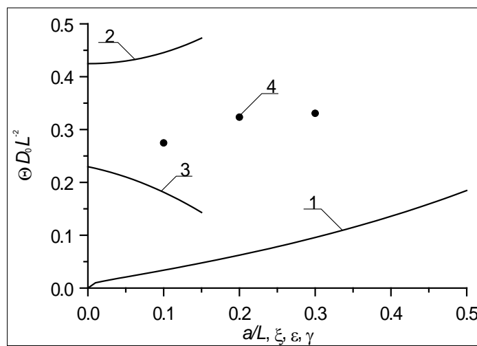
Fig 5a: Dimensionless optimal annealing time of infused dopant as a function of several parameters.
