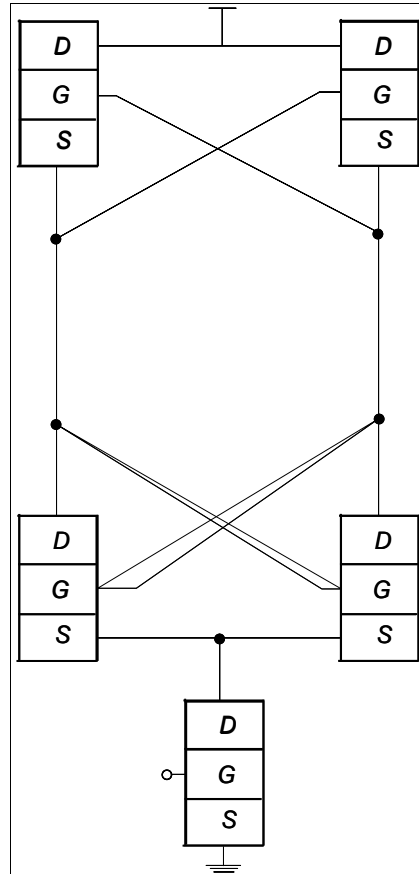
Fig 1: The considered the comparator [4]
