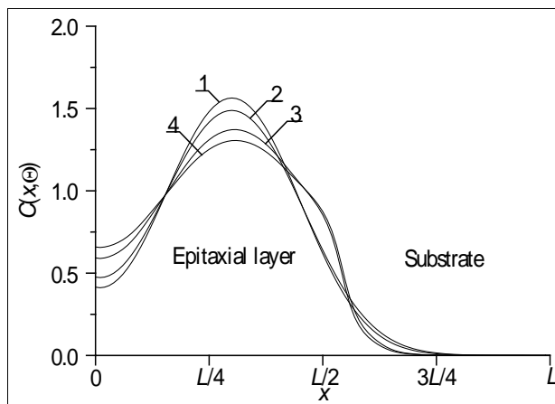
Fig 2b: Dependences of concentration of dopant, implanted in hetero-structure
