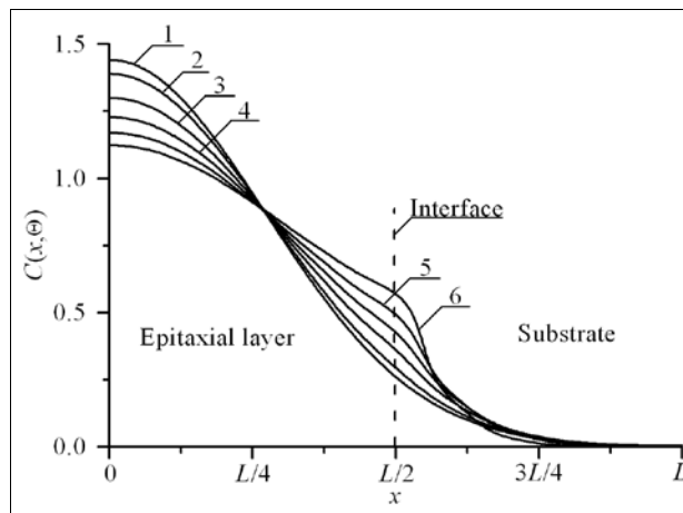
Fig 2a: Dependences of concentration of dopant, infused in hetero-structure
