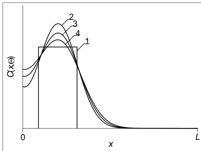
Fig 4b: Distributions of concentration of implanted dopant in depth of hetero-structure
