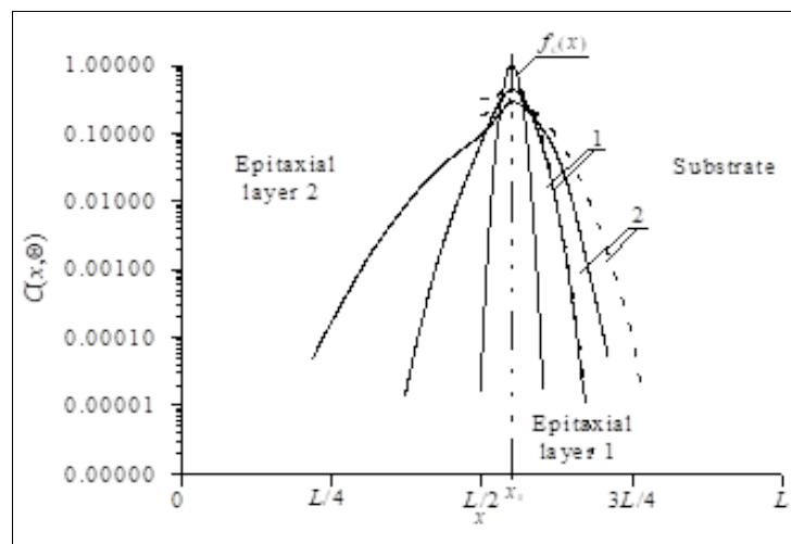
Fig 3b: Calculated distributions of implanted dopant in epitaxial layers of hetero-structure.
