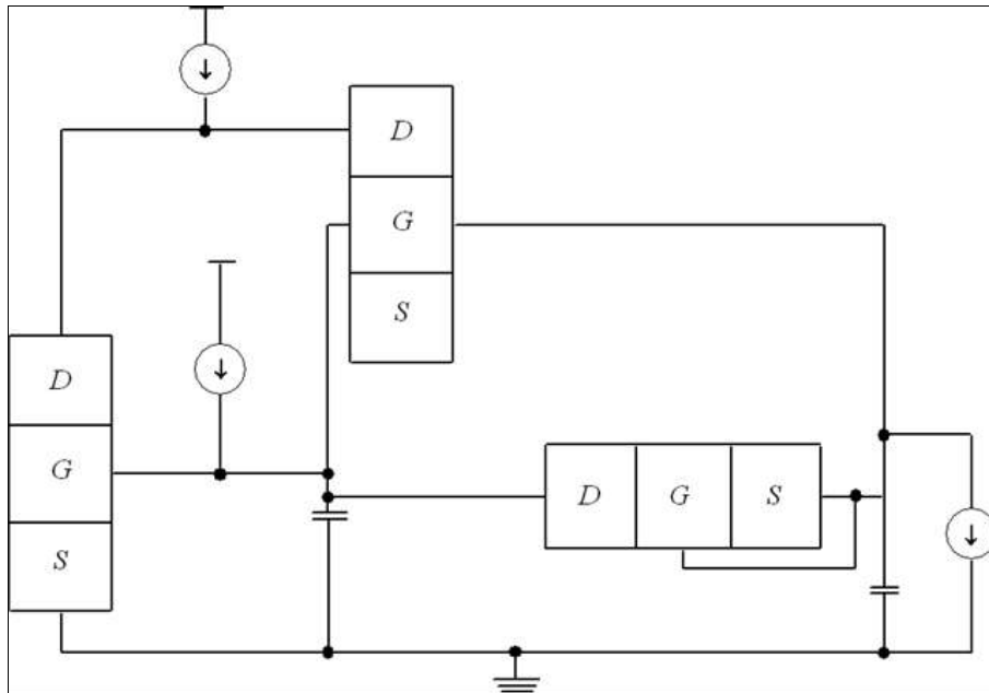
Fig 1a: Structure of the considered filter [15]
