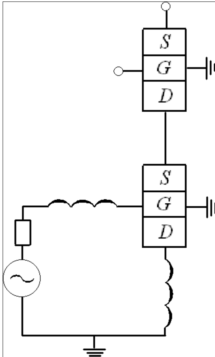
Fig 1A: Structure of the considered cascode amplifier [24]
