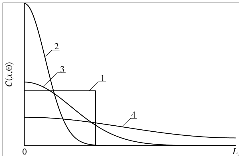
Fig 4a: Distributions of concentration of infused dopant in depth of heterostructure from Fig. 1 for different values of annealing time (curves 2-4) and idealized step-wise approximation (curve 1). Increasing of number of curve corresponds to increasing of annealing time
