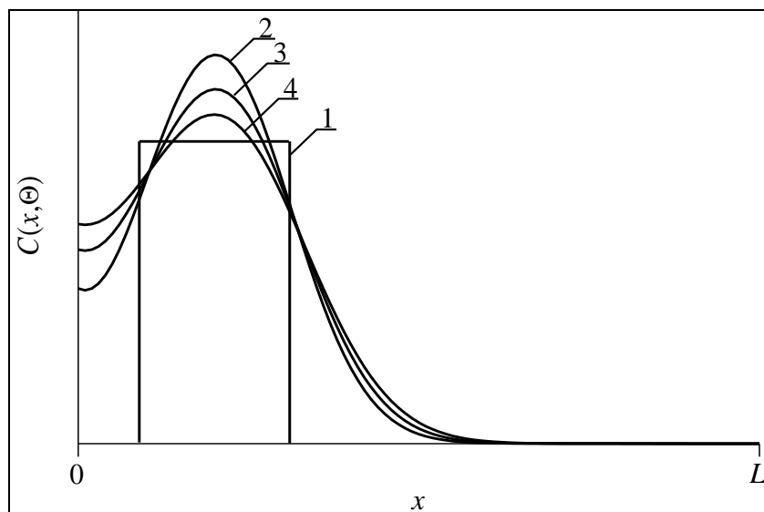
Fig 4b: Distributions of concentration of implanted dopant in depth of heterostructure from Fig. 1 for different values of annealing time (curves 2-4) and idealized step-wise approximation (curve 1). Increasing of number of curve corresponds to increasing of annealing time
