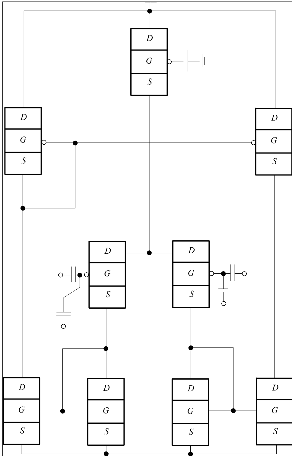
Fig 1: The considered the comparator [4]
