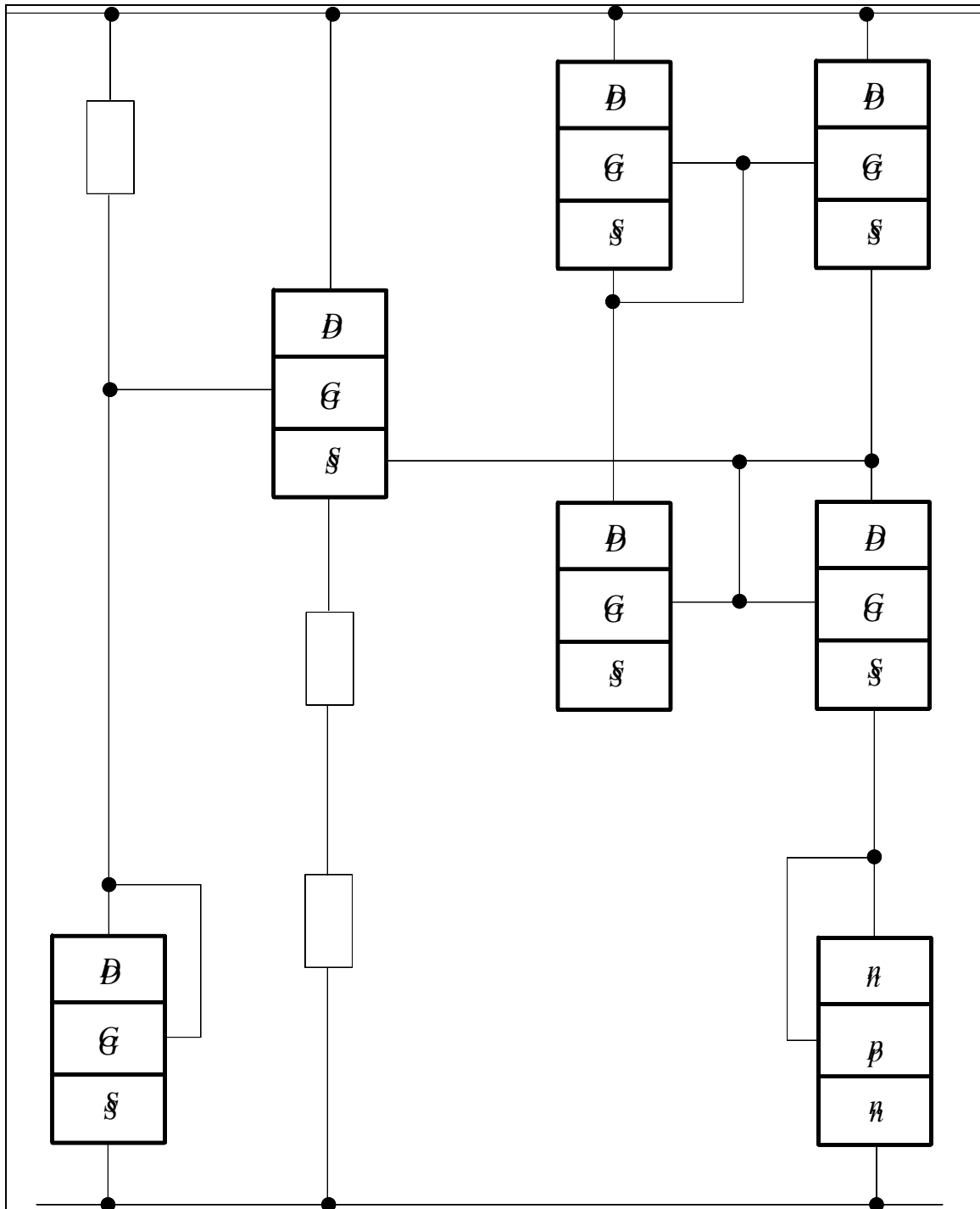
Fig 1a: Structure of the considered amplifier [19]
