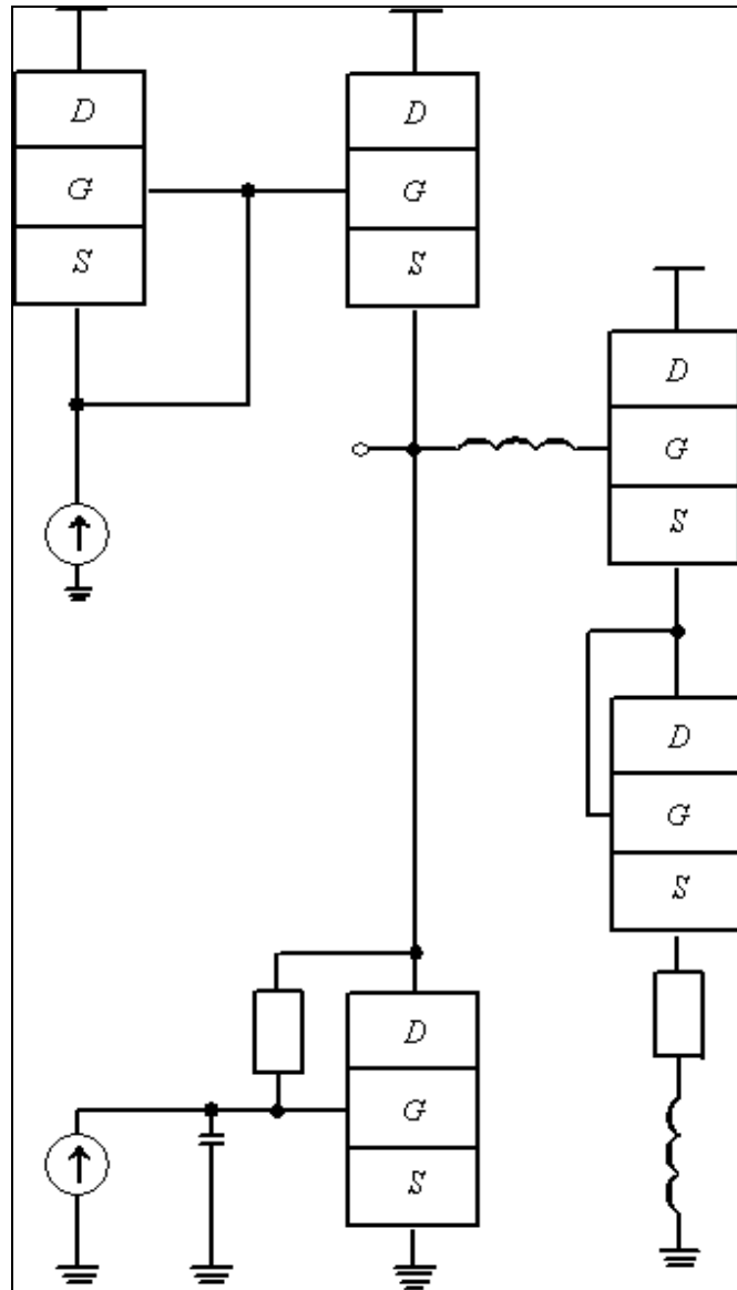
Fig 1a: Structure of the considered amplifier [19]
