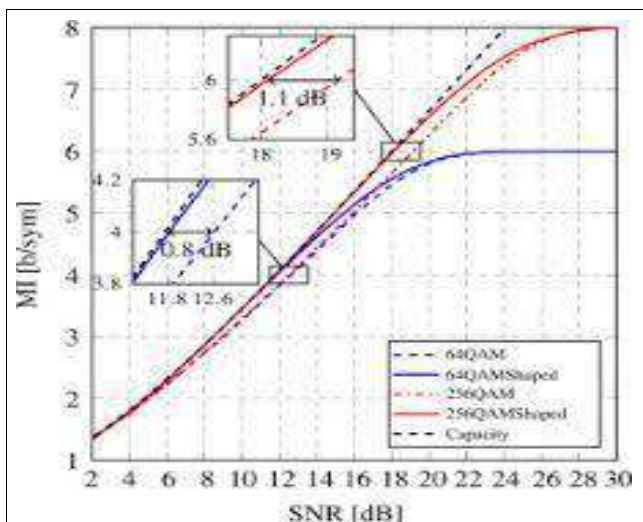
Fig 2: Graph SNR
